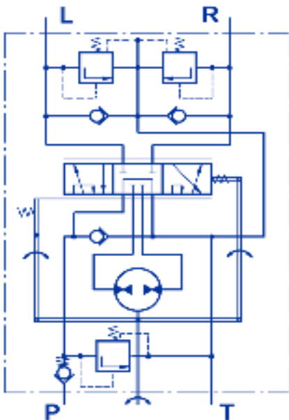
Open center Non Load Reaction with Built-In Valves
